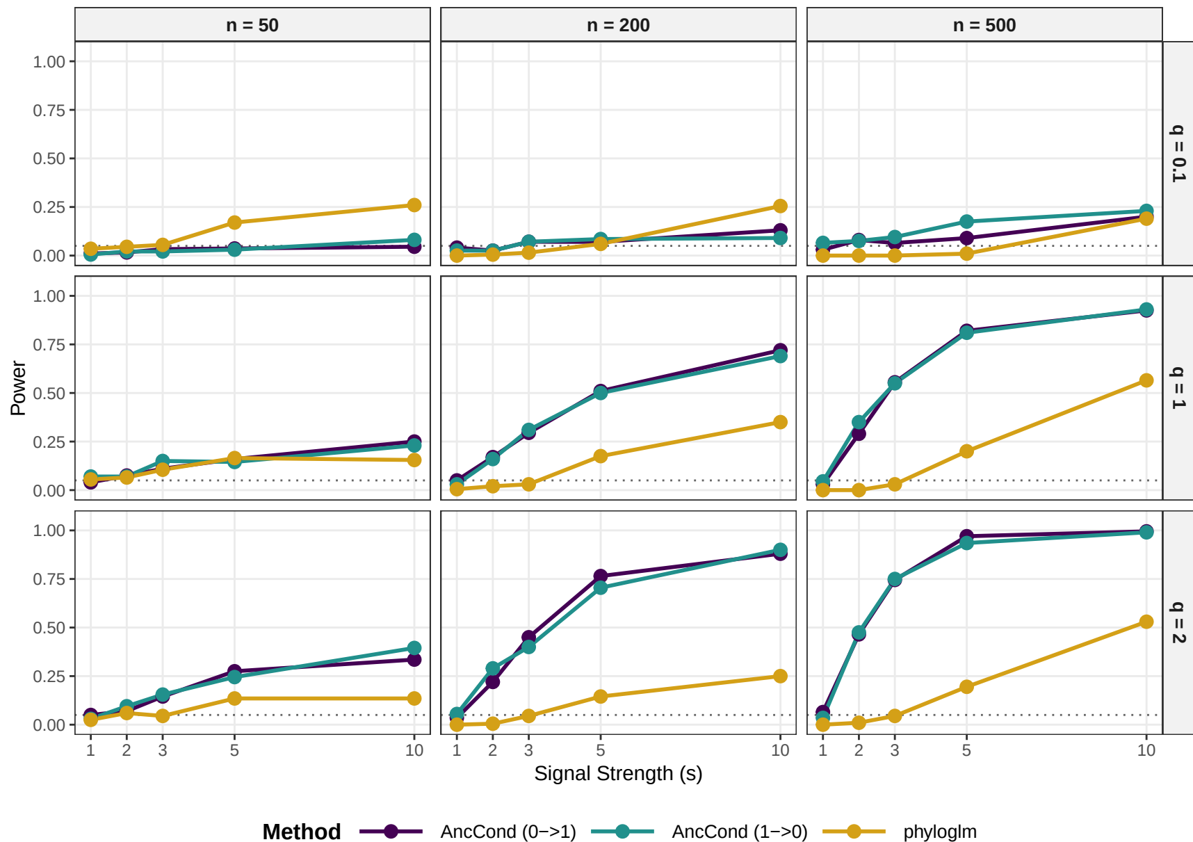
Method Performance: Power Comparison
